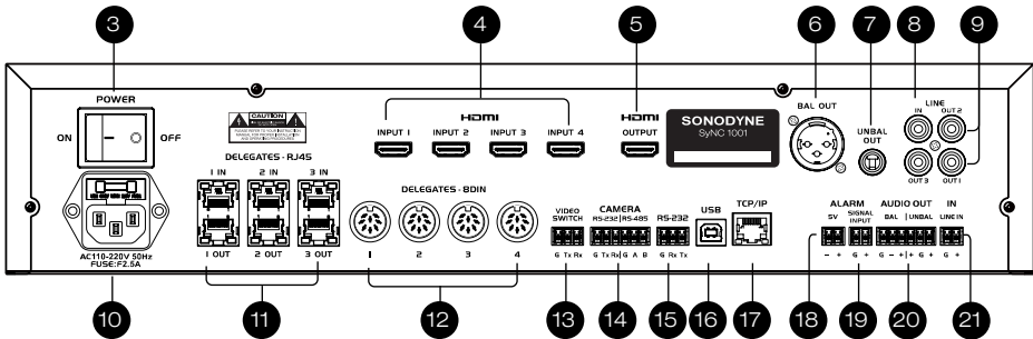
FIG. 2.1b: REAR PANEL
